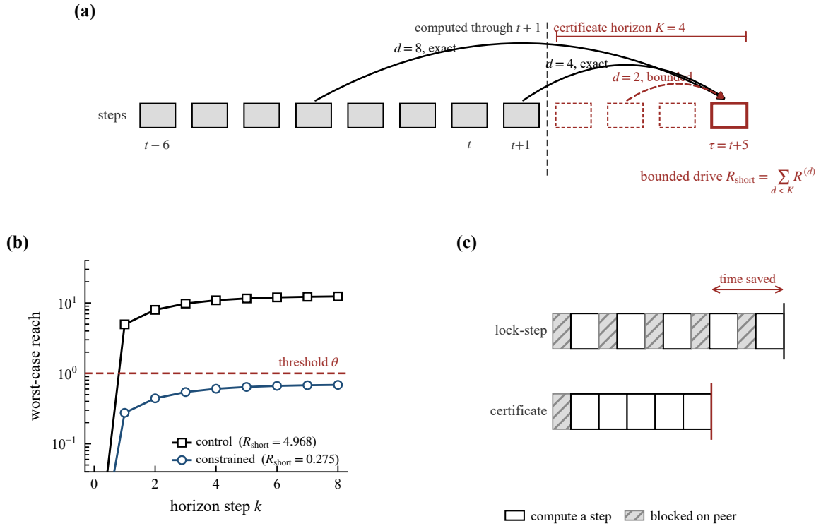
Figure 1. Provable silence from the temporal placement of excitation. (a) A certificate rooted after step t + 1 asks whether step \tau = t + 1 + k can fire. A synapse of delay d supplies that step from \tau - d : for d \geq k this is a step already computed, so its contribution is known exactly, while d < k draws on a step still inside the horizon and must be bounded. With \mathcal{D} = \{2, 4, 8\} and K = 4 only the d = 2 tap is bounded, and the quantity that constrains the certificate is R_{\text{short}} = \sum_{d < K} R^{(d)} . (b) Worst-case membrane reach over the horizon, \beta^k v + R_{\text{short}}(1 - \beta^k)/(1 - \beta) , evaluated at the measured R_{\text{short}} of the control and constrained networks of table 1 with \beta = e^{-1/2} and \theta = 1 . The control exceeds threshold at the first step; the constrained network stays below it for every horizon, which is what the certificate asserts. (c) What a certificate licenses: a core holding one advances through the horizon without waiting for its neighbour, instead of blocking once per step. Schematic; measured timings are in tables 5 and 6.
