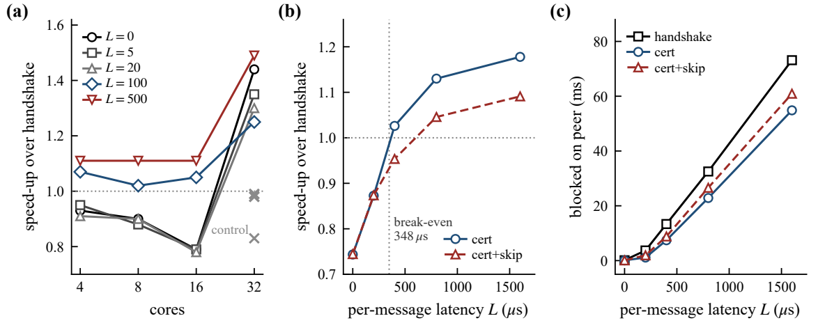
Figure 2. Where barrier-free execution pays. (a) Shared-memory engine: speed-up over lookahead-aware local handshaking against core count, at five emulated latencies; the unconstrained control (crosses, 32 cores) gains nothing at any latency. (b) Two-process TCP engine: speed-up against per-message latency L . Certificates cross unity near the break-even latency at which the waiting they remove equals the computation they add. (c) Time the main loop spends blocked on its peer, the quantity a certificate acts on. Omitting frames from certified-silent ranks stalls longer than transmitting every step, which is why it is slower in (b) despite sending 28% fewer frames.
