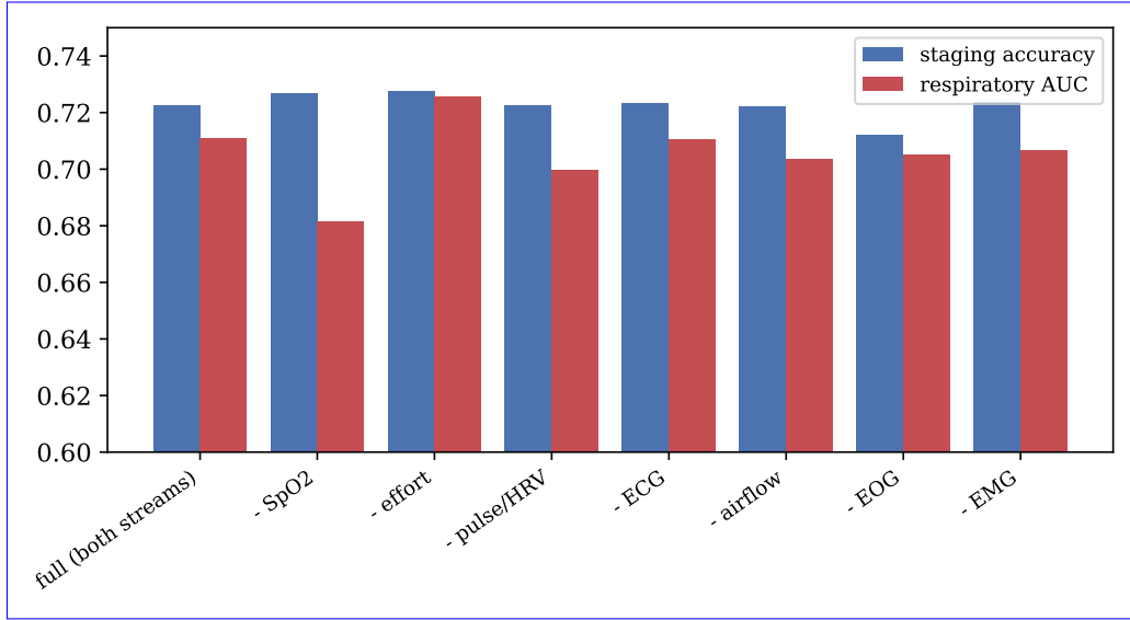
Figure 6: Modality-ablation grid. Staging accuracy (blue) and respiratory AUC (red) as each modality is removed in turn. Removing SpO 2 or the whole cardiorespiratory stream lowers respiratory AUC and leaves staging flat; removing the ocular channel lowers staging.
