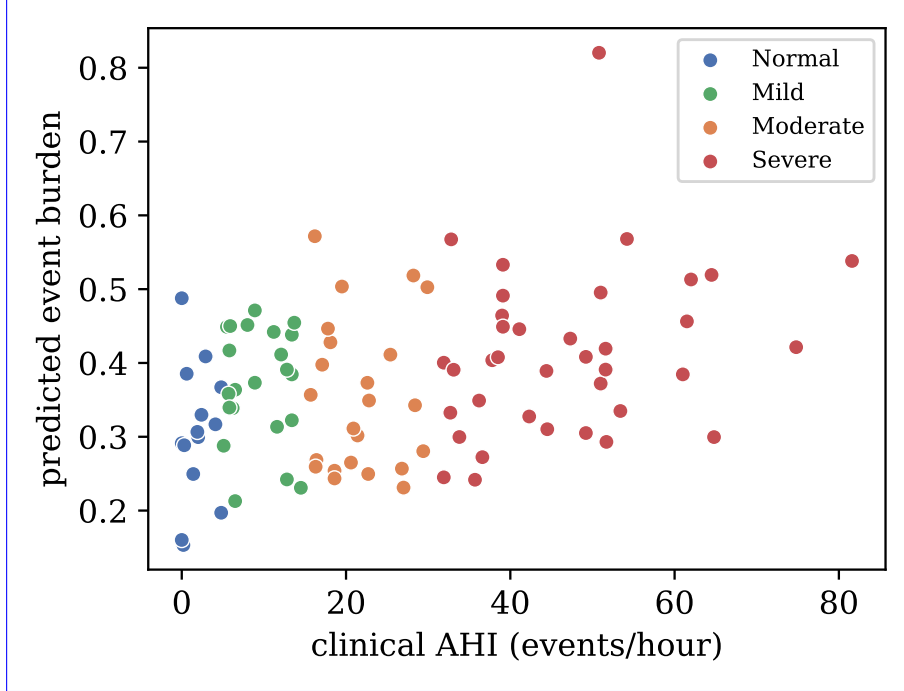
Figure 7: Predicted per-patient event burden (mean respiratory probability) against the clinical apnea-hypopnea index, coloured by AASM severity band. The positive association (Spearman \rho = 0.315 , n = 96 ) shows the model’s output tracks a clinician’s summary measure.
