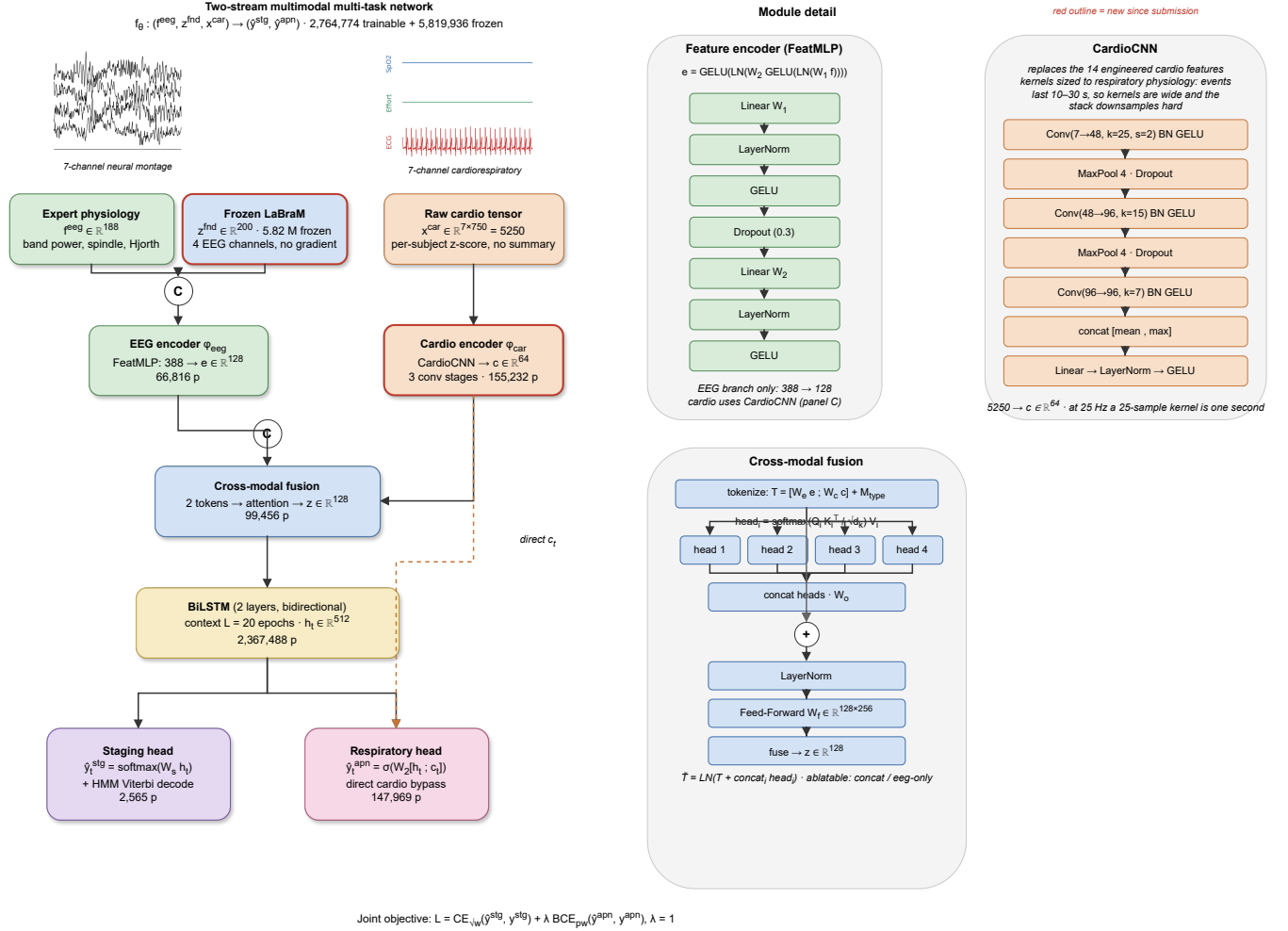
FIGURE 2. The two-stream, multi-task model. (A) The neural features and the cardiorespiratory features are encoded in parallel, combined by a cross-modal fusion block, and read across the night by a bidirectional LSTM. A staging head reads the recurrent state; a respiratory head reads the recurrent state together with a direct copy of the cardiorespiratory embedding, so oxygen-desaturation and effort cues reach the respiratory decision without passing through the staging-oriented fusion. (B) Detail of the feature encoder and of the fusion block, which tokenizes the two modalities, runs four-head attention, and combines the result with a residual connection.
