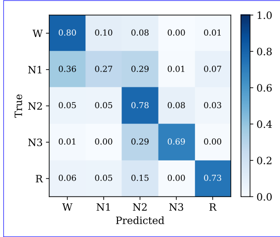
Fig. 4. Row-normalised confusion matrix for the proposed model (pooled ten-fold test epochs, hidden-Markov operating point). Errors concentrate on N1, which is absorbed into Wake and N2.
