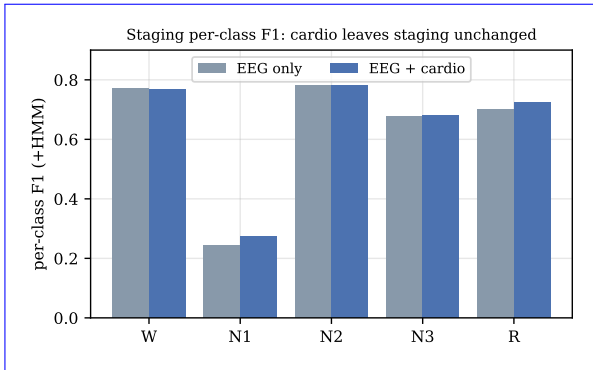
Fig. 5. Per-class staging F1 for the neural-only and the neural-plus-cardiorespiratory model. Adding the cardiorespiratory channels leaves every stage at its full level, including Wake and REM.
