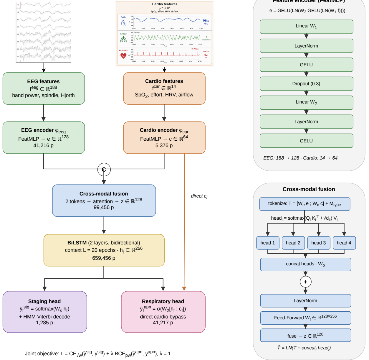
FIGURE 2. The two-stream, multi-task model. (A) The neural features and the cardiorespiratory features are encoded in parallel, combined by a cross-modal fusion block, and read across the night by a bidirectional LSTM. A staging head reads the recurrent state; a respiratory head reads the recurrent state together with a direct copy of the cardiorespiratory embedding, so oxygen-desaturation and effort cues reach the respiratory decision without passing through the staging-oriented fusion. (B) Detail of the feature encoder and of the fusion block, which tokenizes the two modalities, runs four-head attention, and combines the result with a residual connection.
