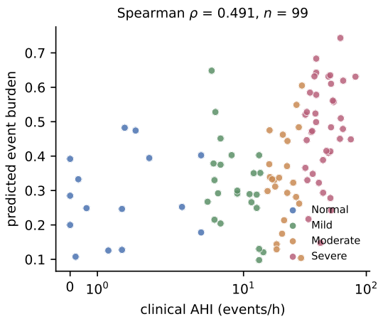
FIGURE 8. [STALE – AHI scatter not yet regenerated for the final model] Predicted per-patient event burden (mean respiratory probability) against the clinical apnea-hypopnea index, coloured by AASM severity band. The positive association (Spearman \rho = 0.491 , n = 99 ) shows the model’s output tracks a clinician’s summary measure.
