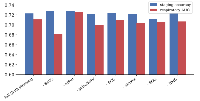
Fig. 6. Modality-ablation grid. Staging accuracy (blue) and respiratory AUC (red) as each modality is removed in turn. Removing SpO 2 or the whole cardiorespiratory stream lowers respiratory AUC and leaves staging flat; removing the ocular channel lowers staging.
