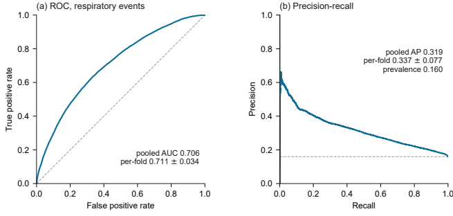
Fig. 7. Respiratory-event detection, operating characteristics, pooled over the ten patient-independent test folds. (a) ROC; the dashed line is chance. (b) Precision–recall; the dashed line is the 0.160 event prevalence, the no-skill floor. Each panel reports the pooled value and the per-fold mean \pm standard deviation, which differ because pooling is a different estimator from cross-validated averaging.
