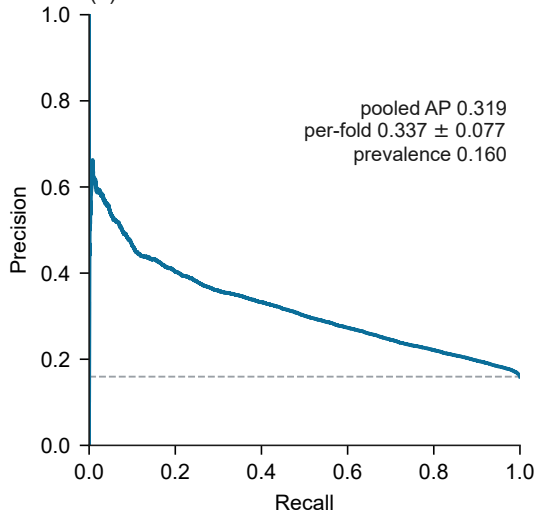
(b) Precision-recall
