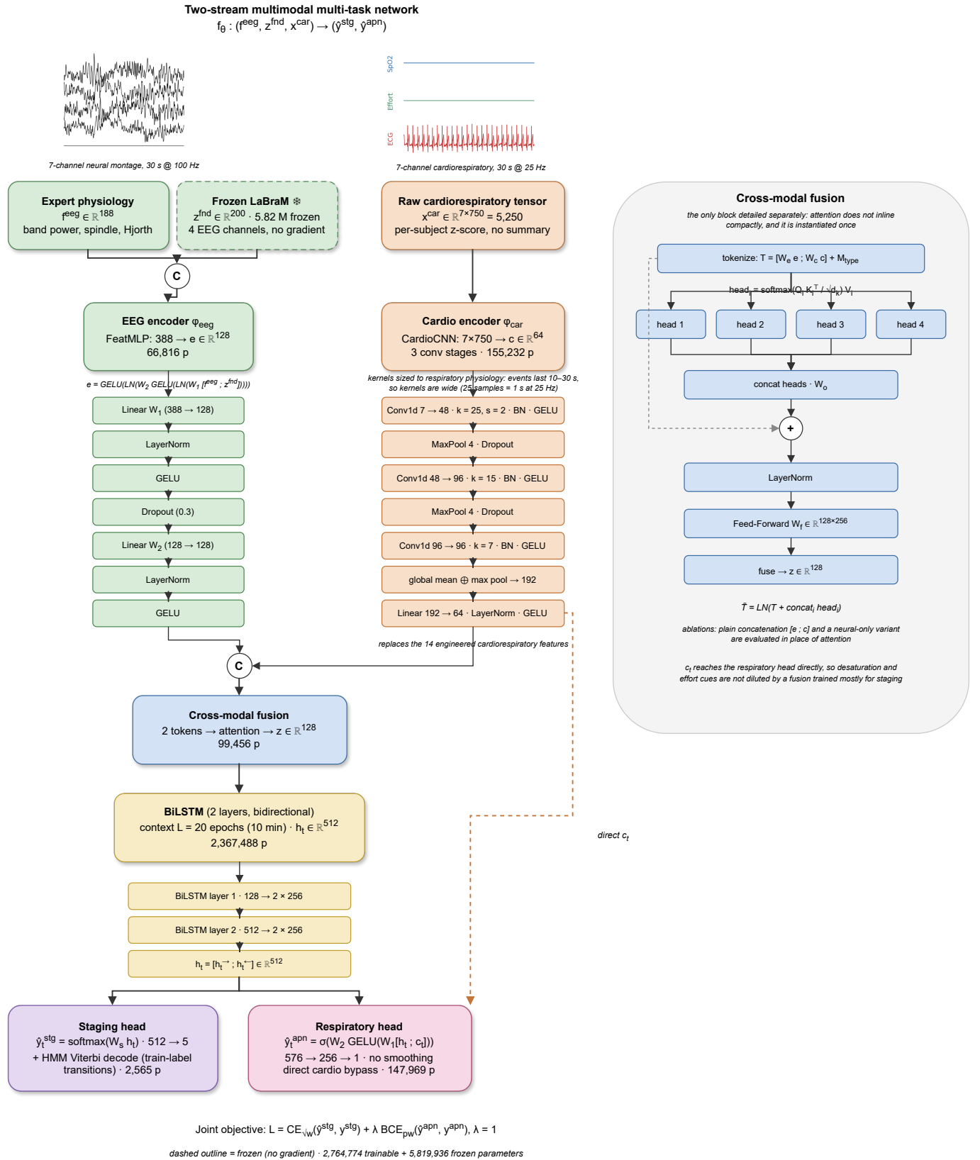
FIGURE 2. The two-stream, multi-task model. Expert physiological features and a frozen self-supervised embedding are concatenated into a 388-dimensional neural input; the cardiorespiratory stream is the raw 7 \times 750 tensor read by a learned convolutional encoder. Both encoders are drawn with their internals expanded, since each is instantiated once. The two embeddings are fused and read across the night by a bidirectional LSTM. A staging head reads the recurrent state; a respiratory head reads it together with a direct copy of the cardiorespiratory embedding, so desaturation and effort cues reach the respiratory decision without passing through the staging-oriented fusion. Cross-modal fusion is the one block detailed separately (right), because attention does not expand compactly in line. Dashed outlines mark frozen parameters.
