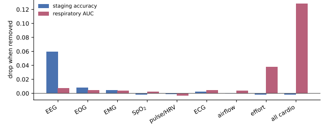
FIGURE 6. Modality-ablation grid. Drop in staging accuracy and in respiratory AUC when each modality is removed and the model retrained.
