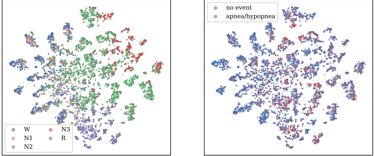
Fig. 10. Two-dimensional t-SNE of the model’s per-epoch embeddings (pooled test epochs). Left: coloured by sleep stage – Wake, N2, N3, and REM form distinct territories while N1 is diffuse. Right: coloured by respiratory-event label – events are spread across the manifold, consistent with the modest detection AUC.
