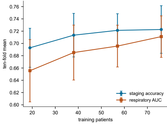
Fig. 9. Learning curve over training-patient fraction, ten-fold patient-independent, error bars one standard deviation across folds. Staging (blue) flattens by 57 patients; respiratory detection (orange) is still climbing at 76.
