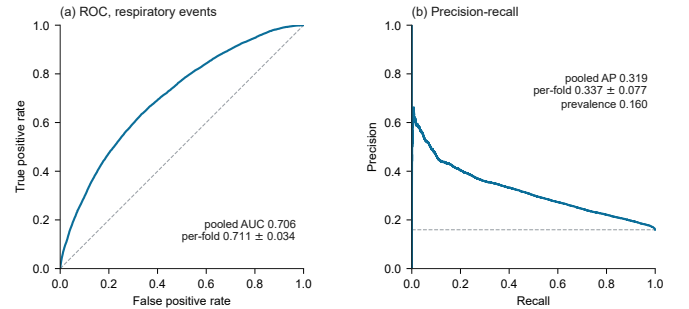
Fig. 7. Respiratory-event detection, operating characteristics, pooled over the ten patient-independent test folds. (a) ROC; the dashed line is chance. (b) Precision–recall; the dashed line is the 0.160 event prevalence, the no-skill floor. Each panel reports the pooled value and the per-fold mean \pm standard deviation, which differ because pooling is a different estimator from cross-validated averaging.
