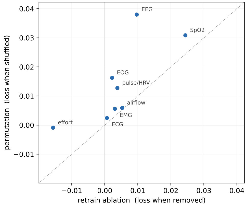
Respiratory AUC Spearman \rho = 0.810 , p = 0.0149^* ( n = 8 )
