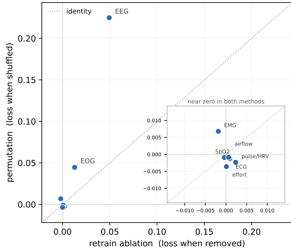
Staging accuracy Spearman \rho = 0.357 , p = 0.3851 ( n = 8 )
