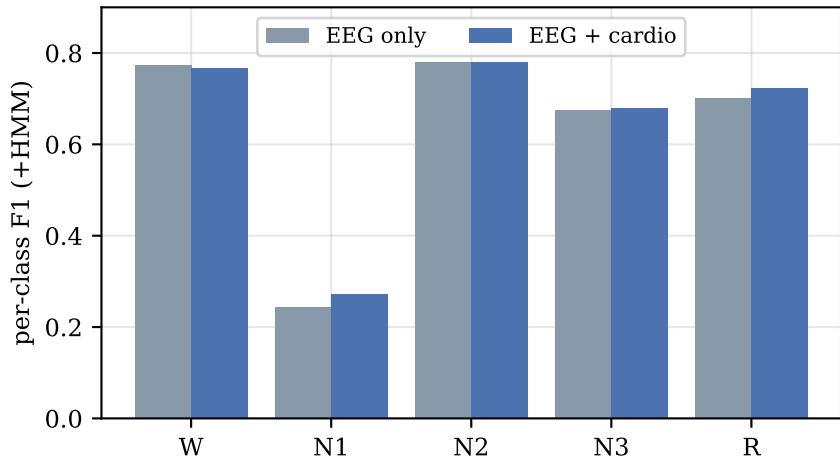
Staging per-class F1: cardio leaves staging unchanged
