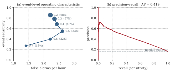
FIGURE 5. Respiratory-event detection, pooled over the ten patient-independent test folds. (a) Event-level operating characteristic. Each point is a decision threshold, labelled and sized by the fraction of all epochs it flags. (b) Precision-recall; the dashed line is the 0.157 event prevalence, the no-skill floor.
