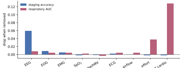
FIGURE 6. Modality-ablation grid. Drop in staging accuracy (blue) and respiratory AUC (red) when each modality is removed and the model retrained.
