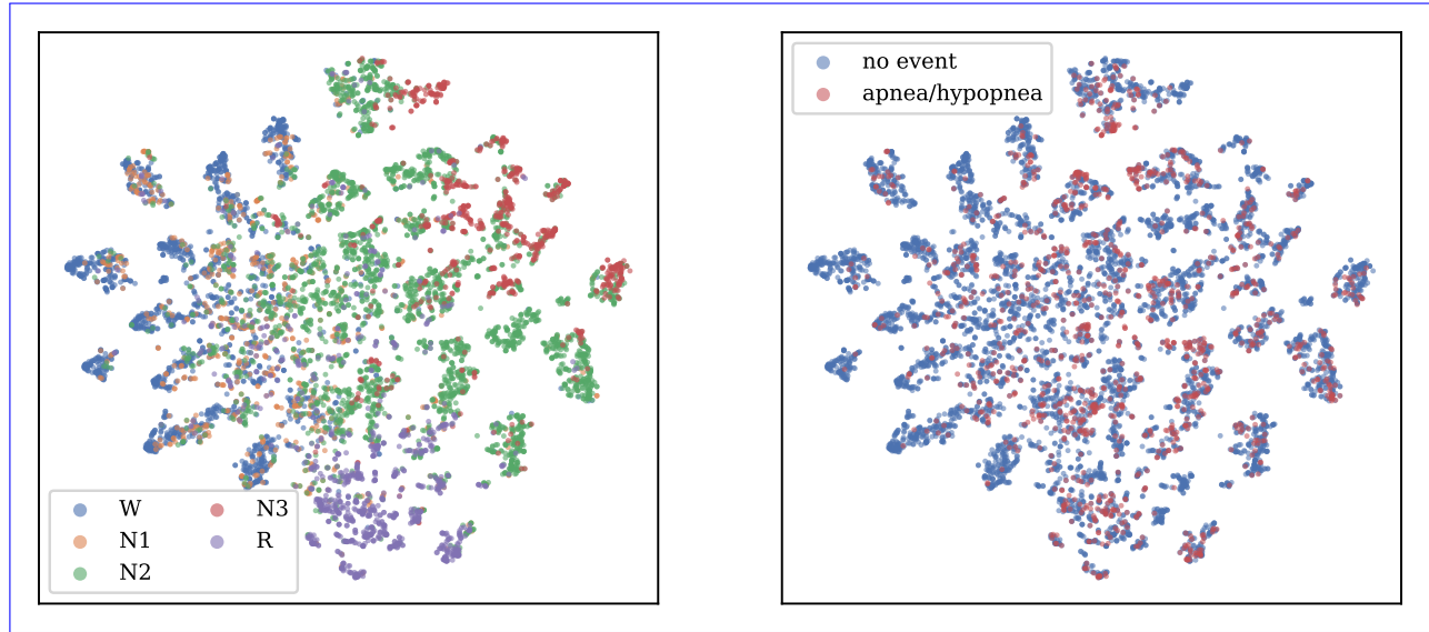
Fig. 8. Two-dimensional t-SNE of the model’s per-epoch embeddings (pooled test epochs). Left: coloured by sleep stage – Wake, N2, N3, and REM form distinct territories while N1 is diffuse. Right: coloured by respiratory-event label – events are spread across the manifold, consistent with the modest detection AUC.
