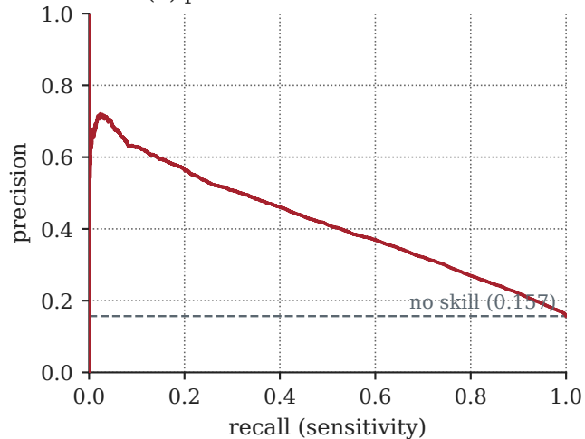
(b) precision--recall AP = 0.419
