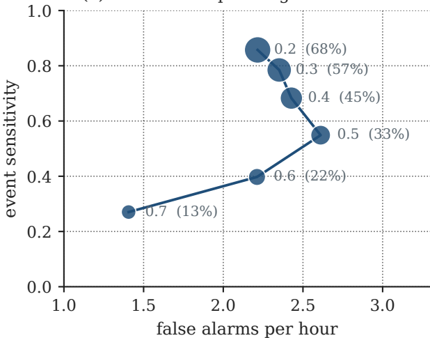
(a) event-level operating characteristic
