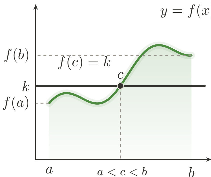
Figure 10.1: Intermediate Value Theorem: a continuous path hits every intermediate height.
