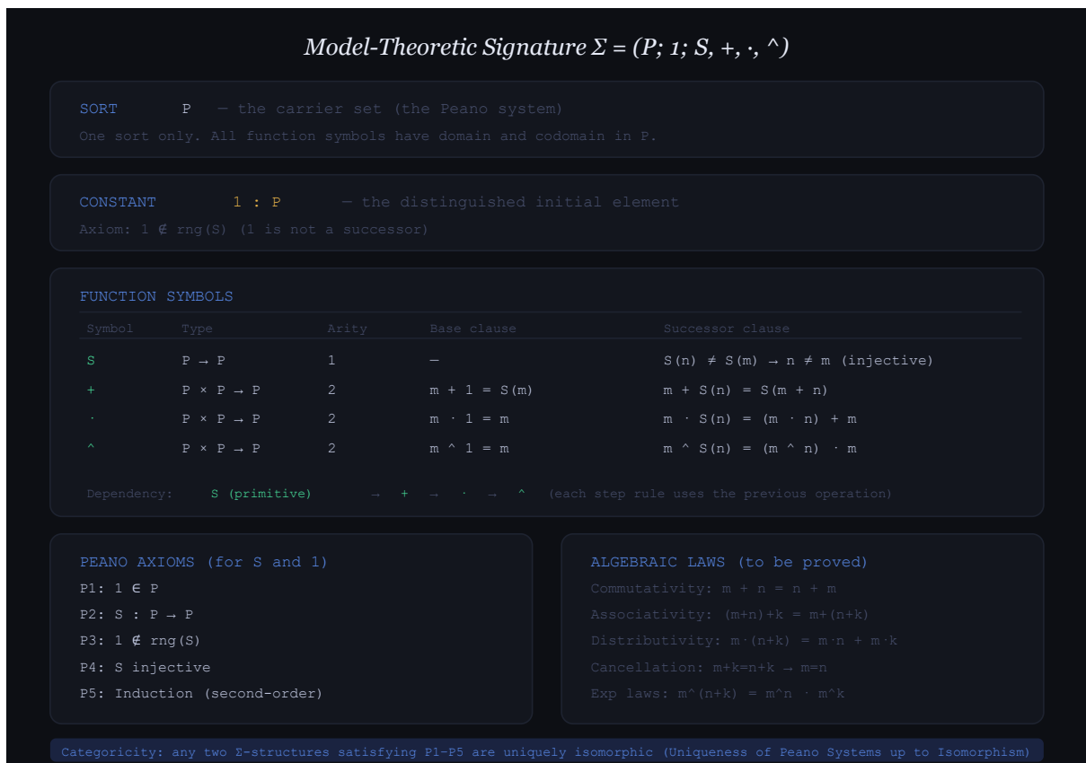
Figure 2.1: The model-theoretic signature for a Peano system and the later arithmetic operations generated from it.
