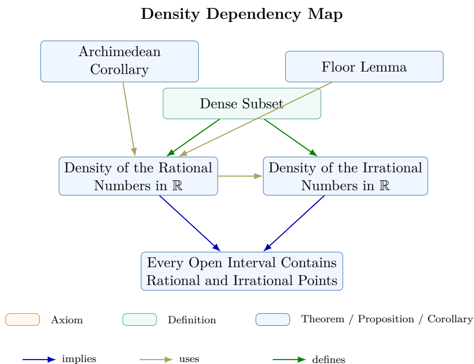
Figure 2.3: Dependency map for the density subchapter. The Floor Lemma and the Archimedean Corollary support the proof of the density of the rational numbers in \mathbb{R} . The irrational density theorem is then derived from the rational density result, and the final corollary combines both density theorems into a single interval statement. The definition records the local vocabulary of the subchapter.
