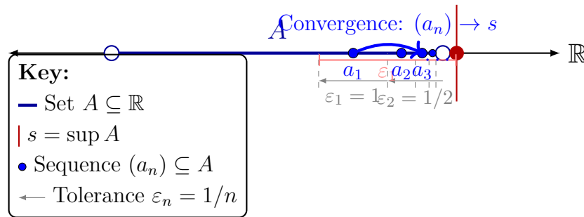
Figure 2.5: Illustrating the constructive connection between the static existence of a supremum ( s ) and the dynamic process of convergence. The \varepsilon -characterization acts as a sequence generator. By selecting decreasing tolerances \varepsilon_n = 1/n , we are guaranteed to find corresponding elements a_n \in A that satisfy s - \frac{1}{n} < a_n \leq s . The sequence (a_n) , contained strictly within A , is forced by the 'squeeze' of the tolerances to converge to s as n \rightarrow \infty . This construction provides the required sequence (a_n) \subseteq A such that \lim_{n \rightarrow \infty} a_n = \sup A .
