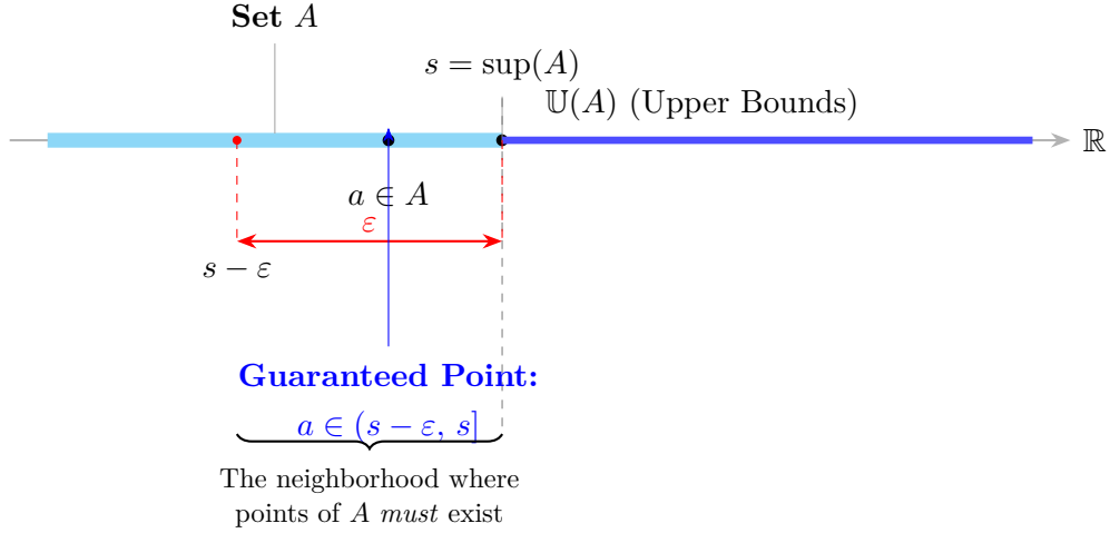
Figure 2.9: Refined visualization of the \varepsilon -characterization. Labels occupy staggered vertical lanes with leader lines to eliminate all horizontal collision, while the dashed spine preserves the geometric correspondence between the real line and the probe below it.
