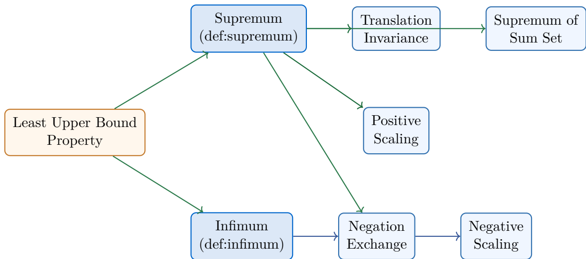
Figure 2.11: Bound Algebra Cluster Dependency Map. The map originates from the ‘Least Upper Bound Property’ (Axiom) and branches into the dual properties of the continuum. The Negation Exchange serves as the structural bridge between supremum and infimum algebra.
