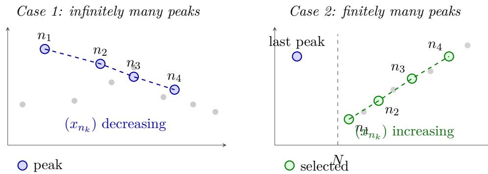
Figure 1.4: The two cases of the Monotone Subsequence Theorem (Section 1.4). Left: Infinitely many peaks (blue) yield a decreasing subsequence (dashed blue). Right: After the last peak, every n \geq N is a non-peak, so a later term always exceeds the current one; this fuels the inductive construction of an increasing subsequence (dashed green).
