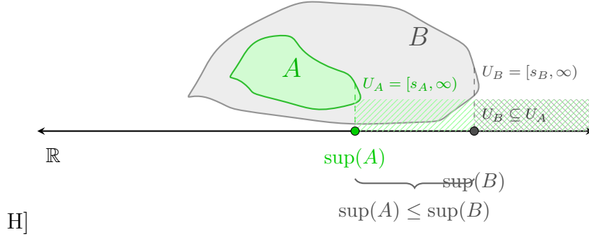
Figure 2.10: The Monotonicity of Supremum Under Set Inclusion. This visualization illustrates the arithmetic consequence of set inclusion, A \subseteq B \subset \mathbb{R} . The topology of the sets is represented by nested blobs where A (green) is contained within B (gray). Vertically dashed projections link the supremal boundary of each set down to the shared real axis, defining the unique points s_A = \sup(A) and s_B = \sup(B) . The figure demonstrates that because the territory of A is restricted by B , its maximum guard point s_A cannot exceed s_B . Finally, the shaded regions illustrate the territories of upper bounds ( U_A and U_B ), clearly showing that U_B is a proper subset of U_A . Any value guarding the larger set B necessarily satisfies the guard condition for the smaller set A .
