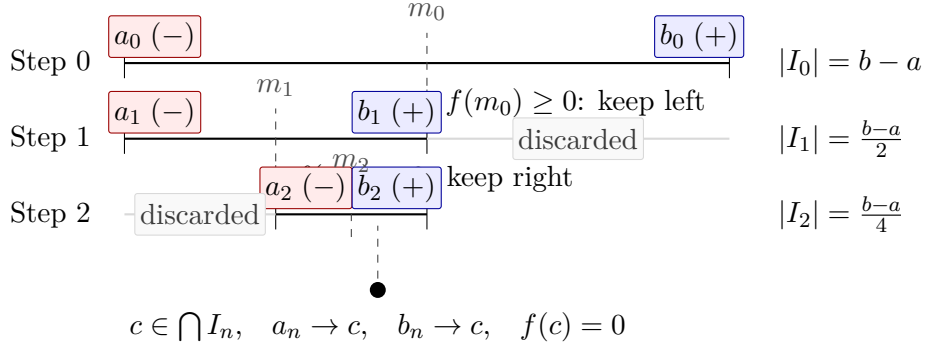
Figure 1.7: Three steps of the bisection proof of the Intermediate Value Theorem (Proposition 1.5.11) for f(a) < 0 < f(b) . At each step the half preserving a sign change is retained and the other discarded; lengths halve as (b-a)/2^n \rightarrow 0 . By NIP, c \in \bigcap I_n exists uniquely; continuity forces f(c) = 0 .
