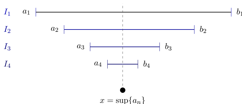
Figure 1.6: The Nested Interval Property (Section 1.6.1). Left endpoints a_n increase; right endpoints b_n decrease; each b_n is an upper bound for \{a_n\} . By the Axiom of Completeness, x = \sup\{a_n\} exists and satisfies a_n \leq x \leq b_n for all n , so x \in \bigcap I_n .
