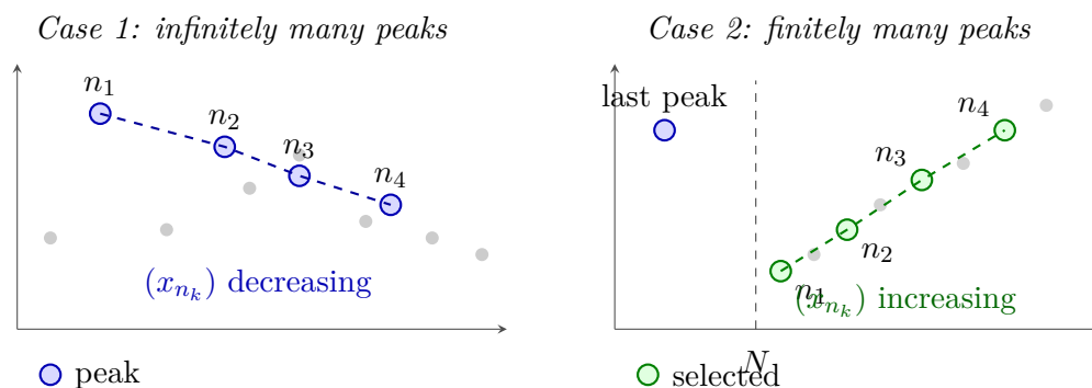
Figure 1.4: The two cases of the Monotone Subsequence Theorem (Section 1.5.3). Left: Infinitely many peaks (blue) yield a decreasing subsequence (dashed blue). Right: After the last peak, every n \geq N is a non-peak, so a later term always exceeds the current one; this fuels the inductive construction of an increasing subsequence (dashed green).
