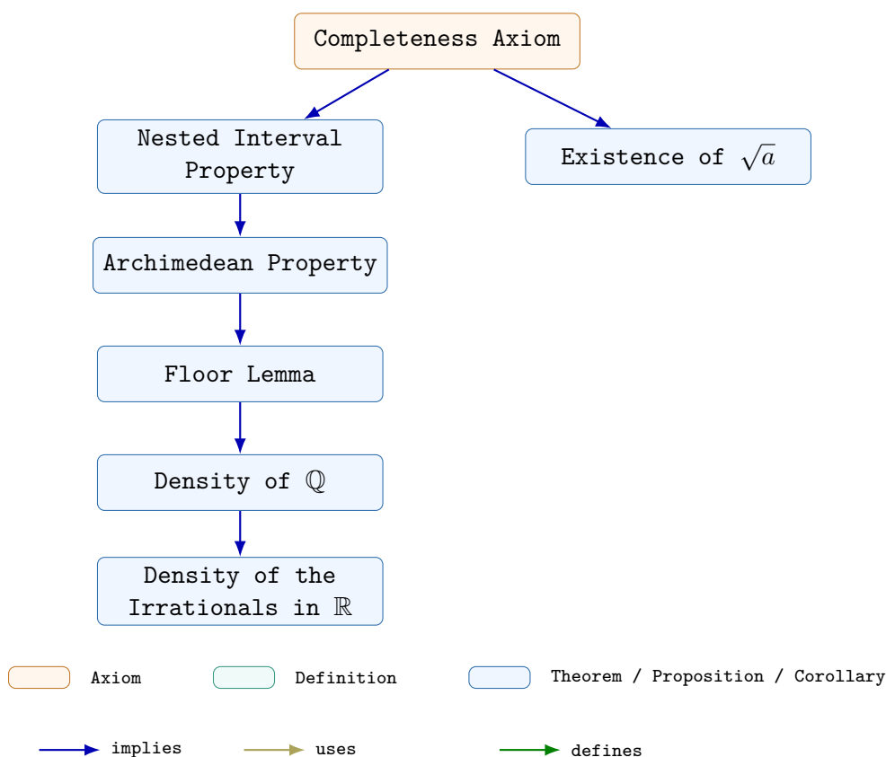
Figure 2.4: Dependency map for the completeness subchapter. The Completeness Axiom yields the Nested Interval Property and the existence of \sqrt{a} ; the Nested Interval Property then supports the Archimedean Property, the Floor Lemma, and the density results for \mathbb{Q} and for the irrational numbers.
