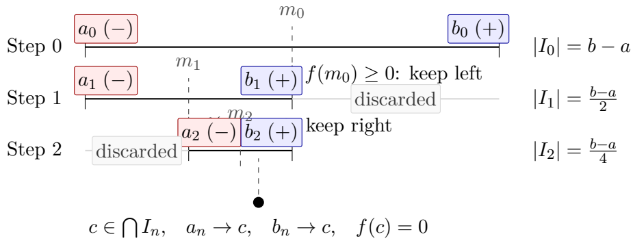
Figure 1.7: Three steps of the bisection proof of the Intermediate Value Theorem (Proposition 1.6.11) for f(a) < 0 < f(b) . At each step the half preserving a sign change is retained and the other discarded; lengths halve as (b - a)/2^n \rightarrow 0 . By NIP, c \in \bigcap I_n exists uniquely; continuity forces f(c) = 0 .
