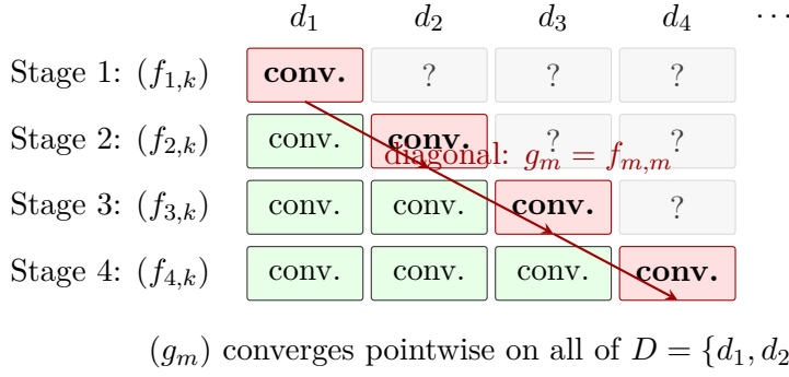
Figure 1.5: Diagonal extraction in the Arzelà-Ascoli argument. Each row (f_{m,k}) converges at d_1, \dots, d_m (green) and is a subsequence of the row above. The diagonal g_m = f_{m,m} (red) is a tail of every row, so it converges at every d_j . Equicontinuity then extends pointwise convergence on the dense set D to uniform convergence on [a, b] .
