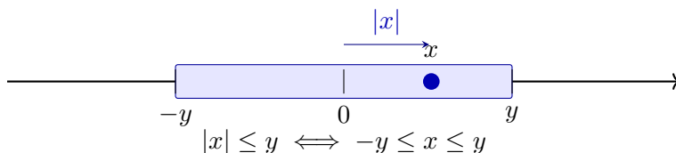
Figure 29.1: The absolute value characterisation as a symmetric interval. The shaded region is [-y, y] ; the point x lies inside with |x| \leq y . The equivalence |x| \leq y \Leftrightarrow -y \leq x \leq y (Proposition 29.1.27(iv)) converts an absolute value bound into a two-sided linear constraint.
