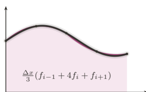
FIGURE 2. Simpson's Rule: Parabolas: Exact to Degree 3
