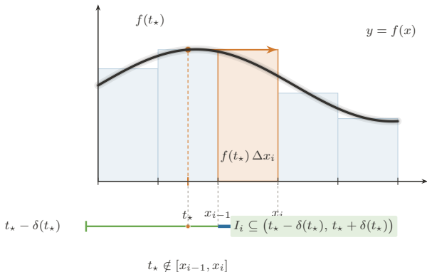
FIGURE. THE MCSHANE INTEGRAL — THE UNTETHERED TAG: A \delta -FINE
