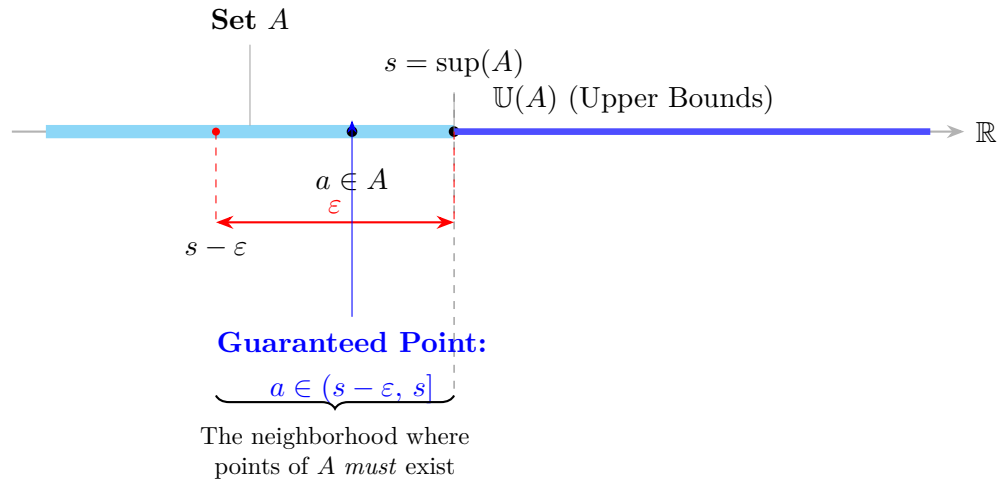
Figure 3.8: Refined visualization of the \varepsilon -characterization. Labels occupy staggered vertical lanes with leader lines to eliminate all horizontal collision, while the dashed spine preserves the geometric correspondence between the real line and the probe below it.
