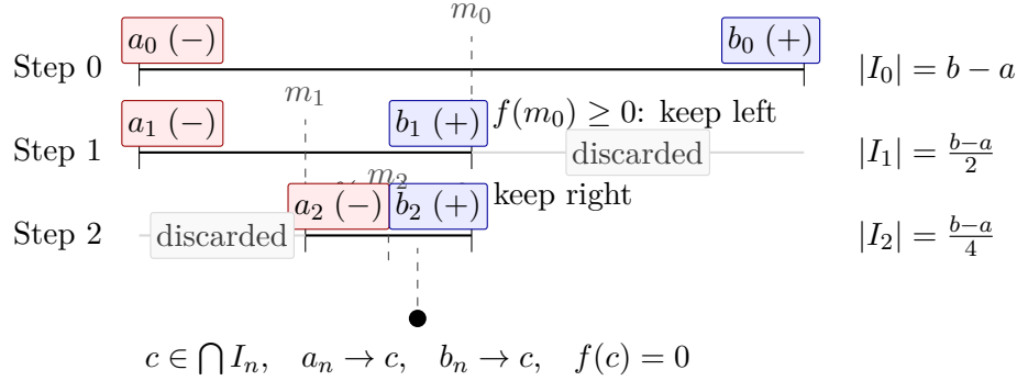
Figure 1.7: Three steps of the bisection proof of the Intermediate Value Theorem ( Proposition 1.1.105 ) for f(a) < 0 < f(b) . At each step the half preserving a sign change is retained and the other discarded; lengths halve as (b - a)/2^n \rightarrow 0 . By NIP, c \in \bigcap I_n exists uniquely; continuity forces f(c) = 0 .
