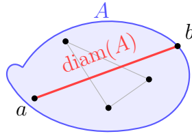
Figure 42.2: The diameter of A is the supremum of the pairwise distances between points of A .
