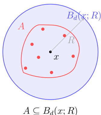
Figure 42.6: An arbitrary subset A of a metric space is bounded when all of its points lie within one finite distance bound from a chosen center.
