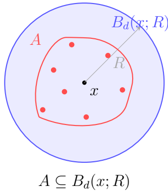
Figure 2.6: An arbitrary subset A of a metric space is bounded when all of its points lie within one finite distance bound from a chosen center.
