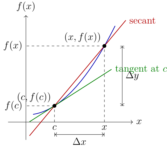
Figure 10.1: The secant line through (c, f(c)) and (x, f(x)) has slope \Delta y/\Delta x . As x \rightarrow c , the secant line rotates toward the tangent line at (c, f(c)) , whose slope is f'(c) .
