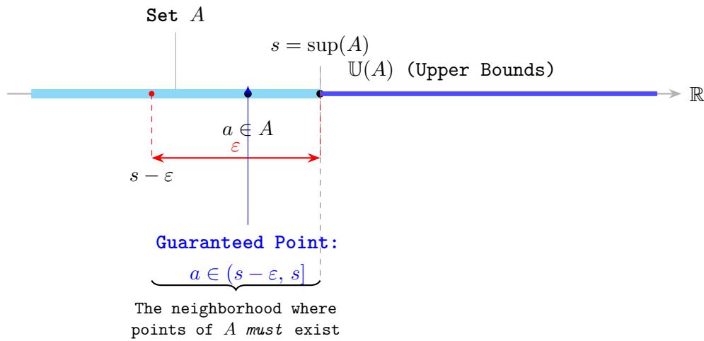
Figure 2.7: Refined visualization of the \varepsilon -characterization. Labels occupy staggered vertical lanes with leader lines to eliminate all horizontal collision, while the dashed spine preserves the geometric correspondence between the real line and the probe below it.
