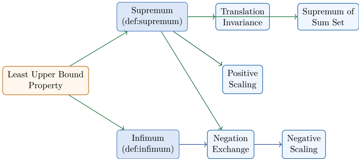
Figure 3.9: Bound Algebra Cluster Dependency Map. The map originates from the ‘Least Upper Bound Property’ (Axiom) and branches into the dual properties of the continuum. The Negation Exchange serves as the structural bridge between supremum and infimum algebra.
