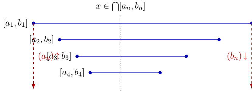
Figure 2.1: Nested intervals [a_1, b_1] \supseteq [a_2, b_2] \supseteq \cdots pinch toward a common point. The sequence of left endpoints is increasing and bounded above; its supremum x lies in every interval.
