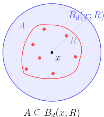
Figure 2.6: An arbitrary subset A of a metric space is bounded when all of its points lie within one finite distance bound from a chosen center.
