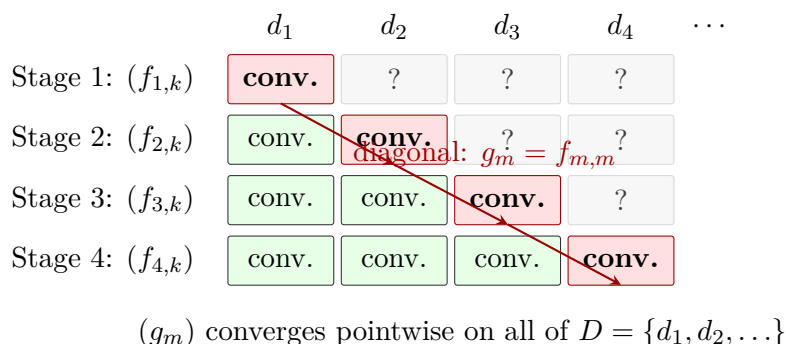
Figure 29.5: Diagonal extraction in the Arzelà–Ascoli argument. Each row (f_{m,k}) converges at d_1, \dots, d_m (green) and is a subsequence of the row above. The diagonal g_m = f_{m,m} (red) is a tail of every row, so it converges at every d_j . Equicontinuity then extends pointwise convergence on the dense set D to uniform convergence on [a, b] .
