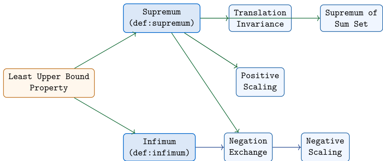
Figure 2.9: Bound Algebra Cluster Dependency Map. The map originates from the ‘Least Upper Bound Property’ (Axiom) and branches into the dual properties of the continuum. The Negation Exchange serves as the structural bridge between supremum and infimum algebra.
