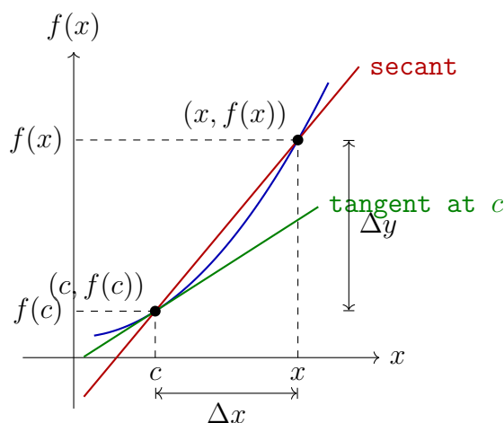
Figure 7.1: The secant line through (c, f(c)) and (x, f(x)) has slope \Delta y / \Delta x . As x \rightarrow c , the secant line rotates toward the tangent line at (c, f(c)) , whose slope is f'(c) .
