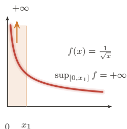
FIGURE 3. Unbounded Integrand: Boundedness Is Not Optional
