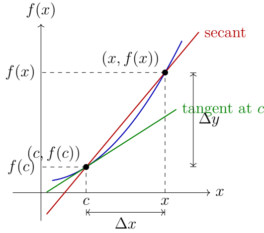
Figure 9.1: The secant line through (c, f(c)) and (x, f(x)) has slope \Delta y / \Delta x . As x \rightarrow c , the secant line rotates toward the tangent line at (c, f(c)) , whose slope is f'(c) .
