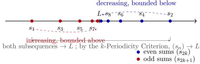
Figure 1.9: Even and odd partial sums of an alternating series \sum(-1)^{n+1}a_n with (a_n) positive, decreasing, and tending to zero. Even sums (s_{2k}) (blue) decrease and are bounded below; by MCT they converge to L . Odd sums (s_{2k+1}) (red) satisfy s_{2k+1} = s_{2k} + a_{2k+1} \rightarrow L . Since both residue classes (mod k = 2 ) converge to L , the k -Periodicity Criterion ( Section 1.6 ) gives (s_n) \rightarrow L .
