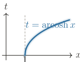
FIGURE HI2. Inverse hyperbolic cosine:
