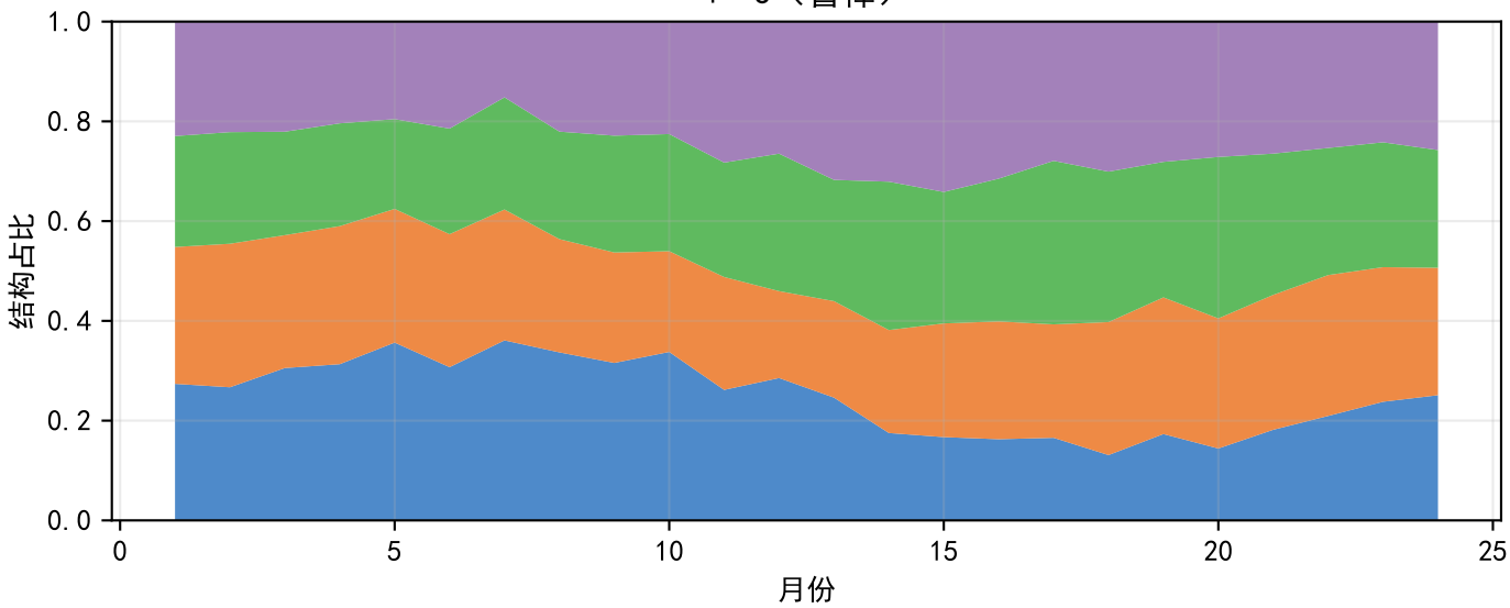
\Gamma=3 (鲁棒)
