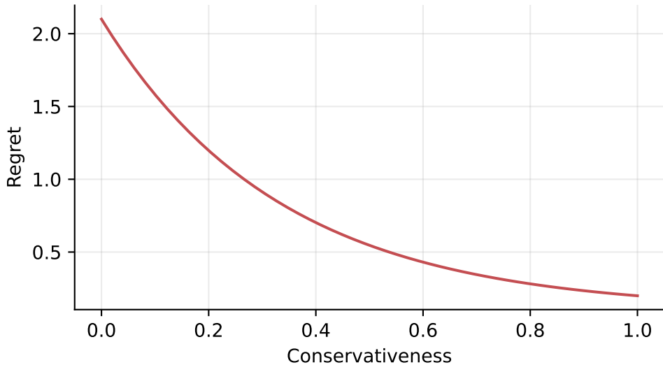
Regret Curve
