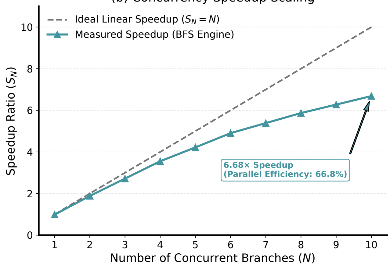
(b) Concurrency Speedup Scaling
