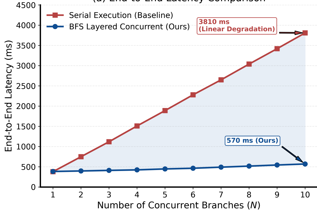
(a) End-to-End Latency Comparison
