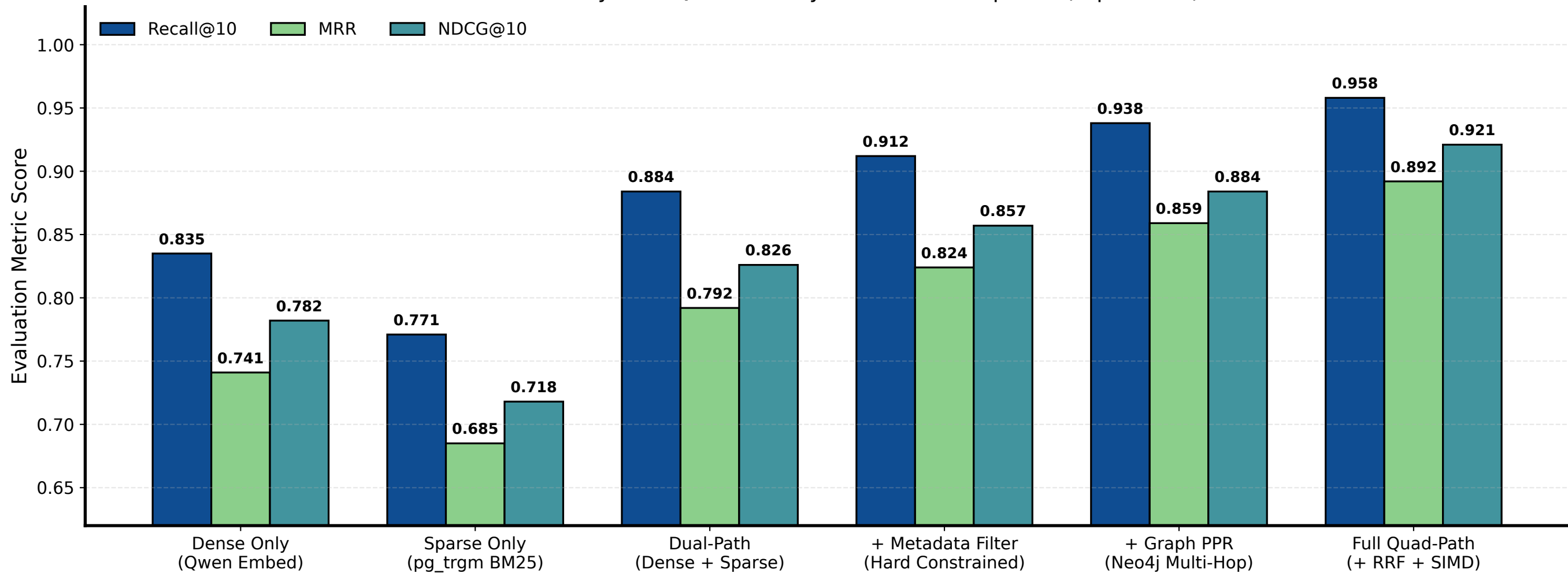
Ablation Analysis of Quad-Path Hybrid Retrieval Pipeline (Top-K = 10)
