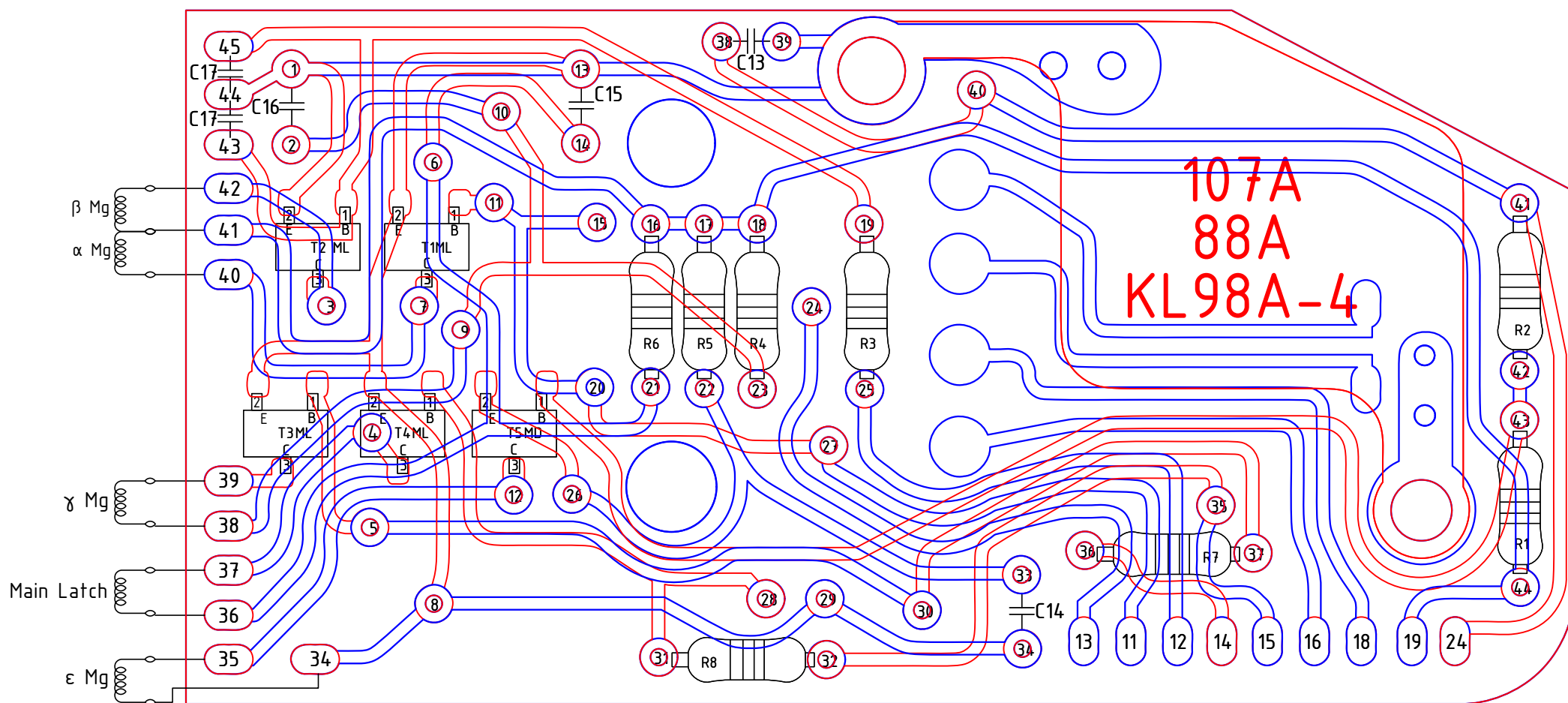
2-64 110a2033630 M-circuit board assembly
