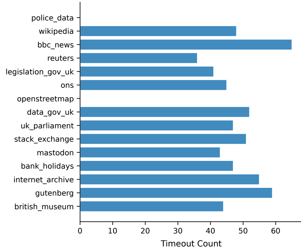
Adapter Timeouts
