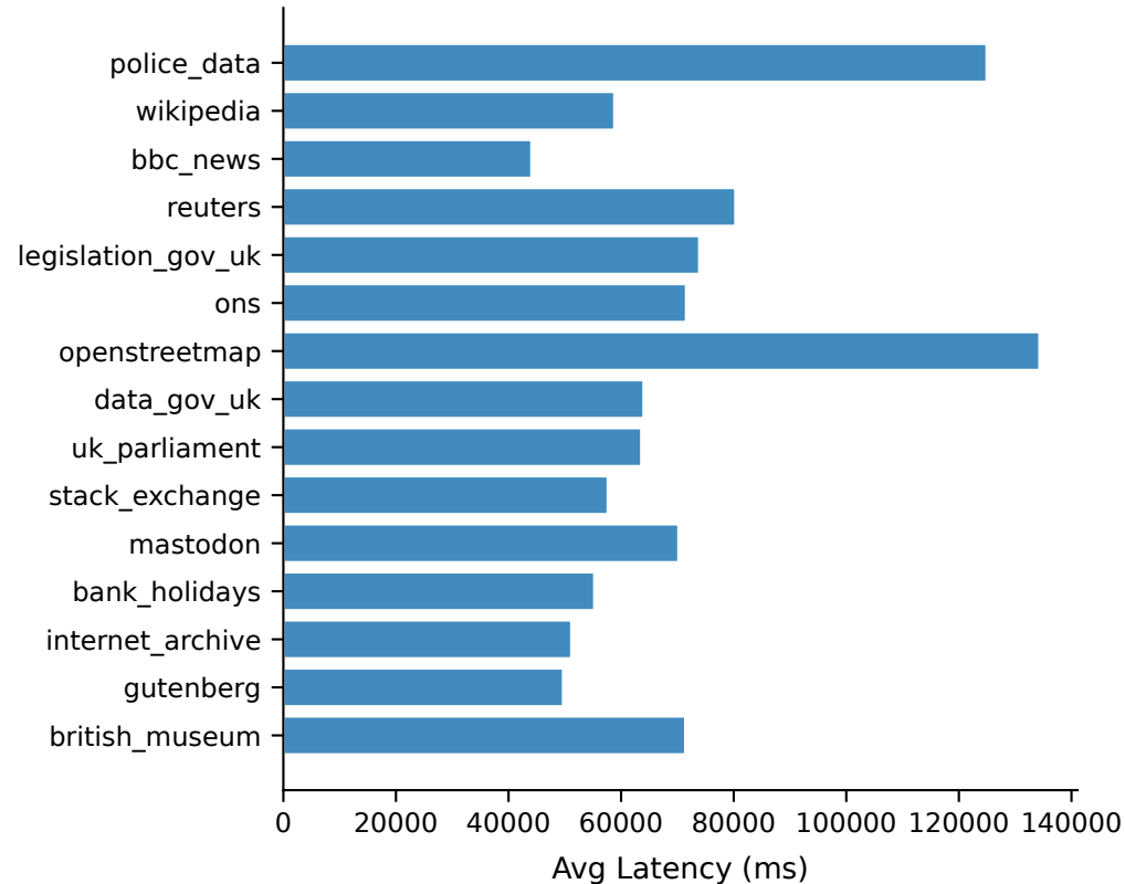
Adapter Latency
