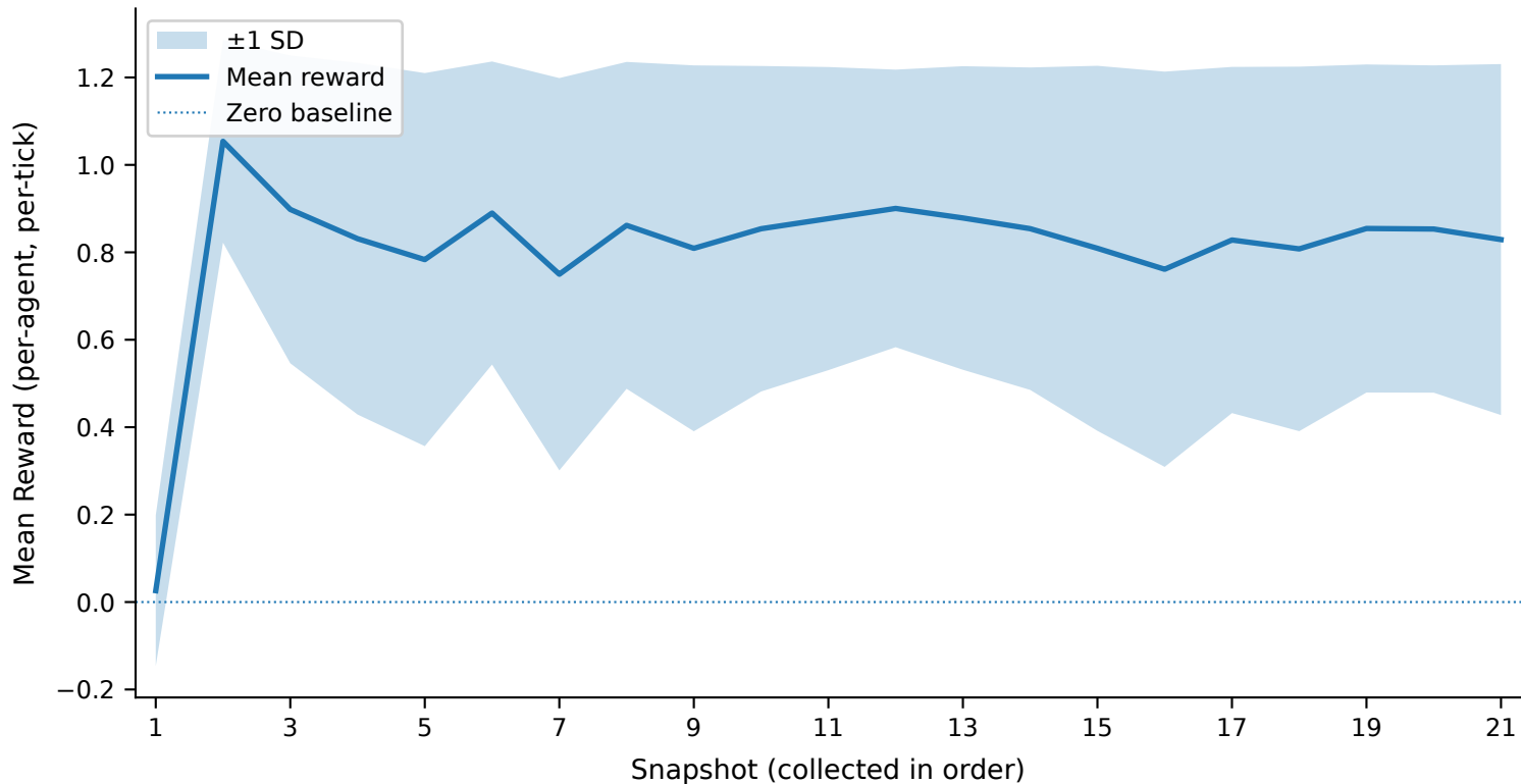
Reward Trajectory
