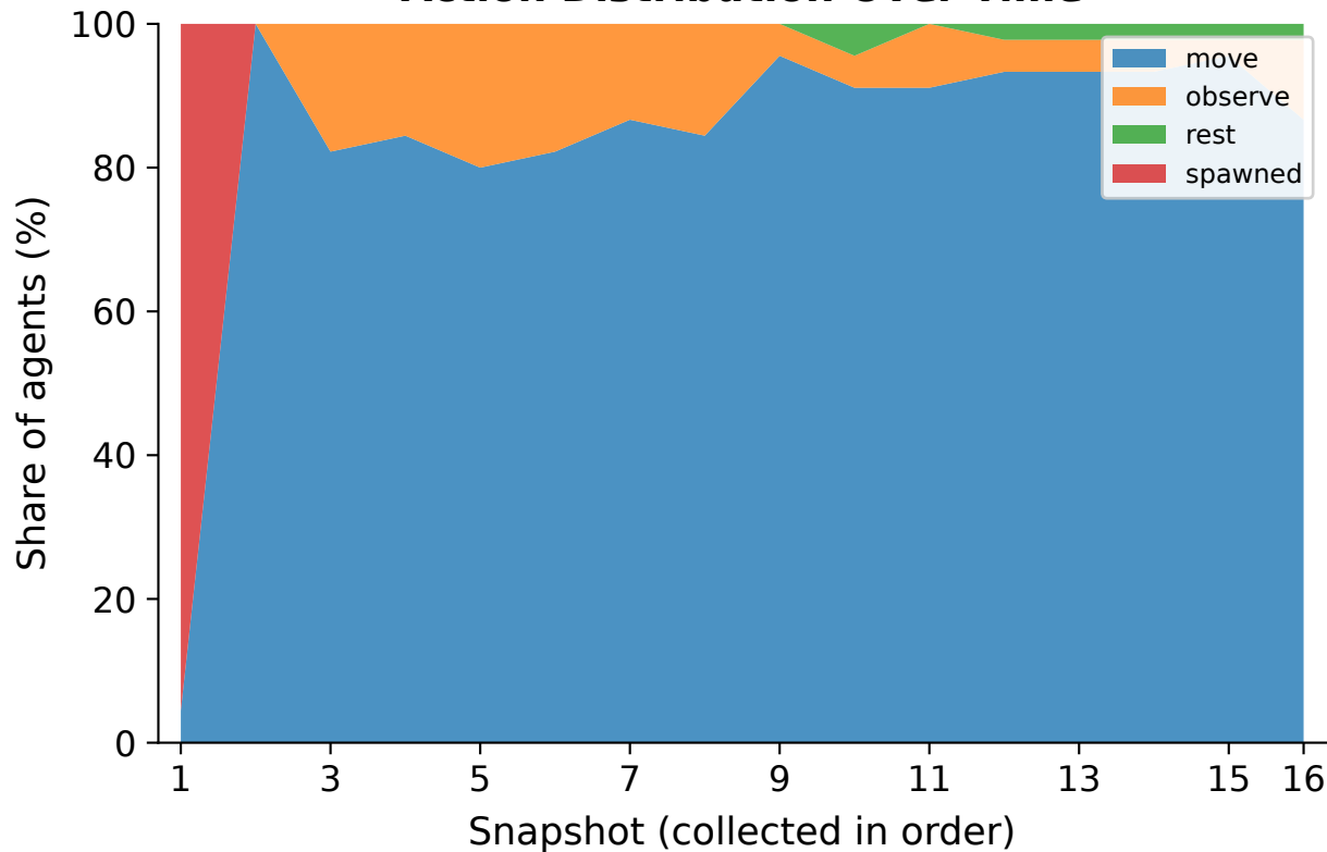
Action Distribution Over Time
