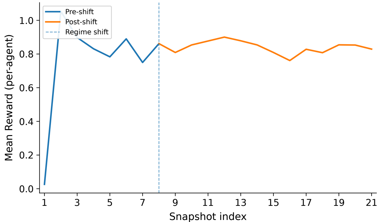
step_change_20: Reward Across Regime Shift
