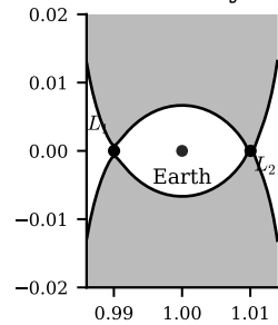
Sun-Earth System
