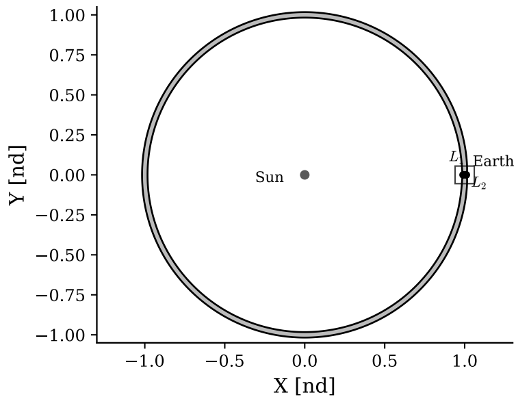
(a) Sun-Earth System
