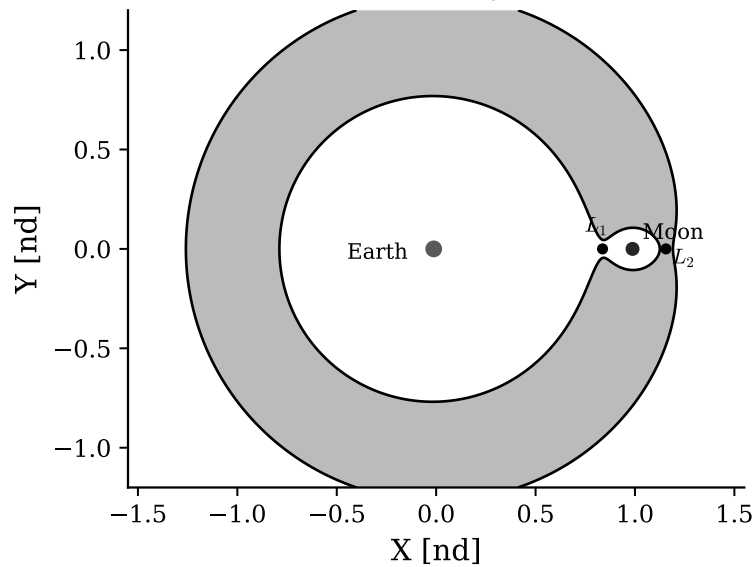
Earth-Moon System
