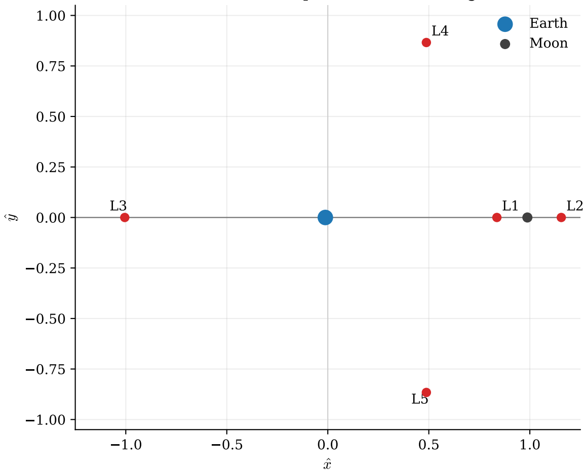
Earth-Moon libration points in the rotating frame
