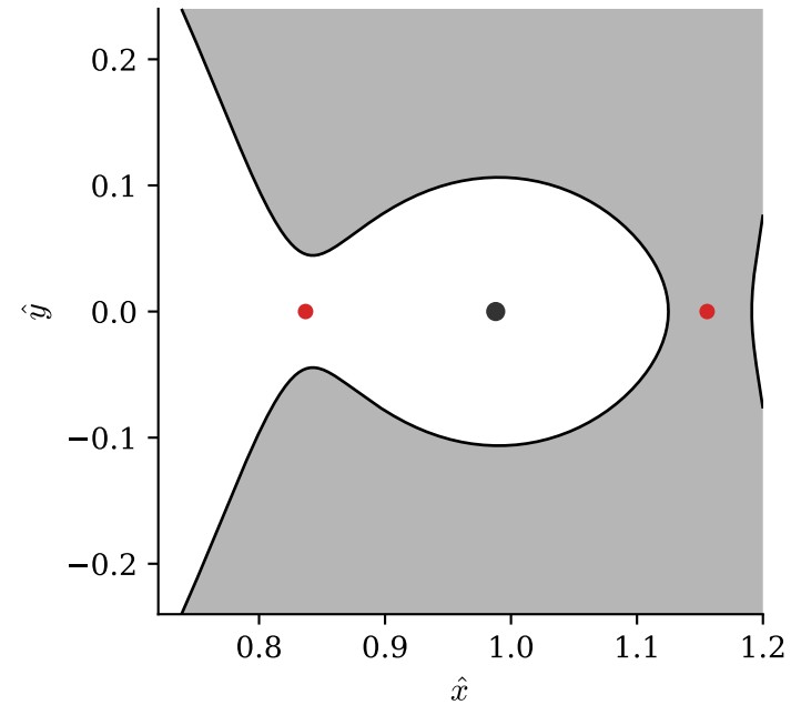
Earth-Moon \mu=0.01215 , JC=3.180251
