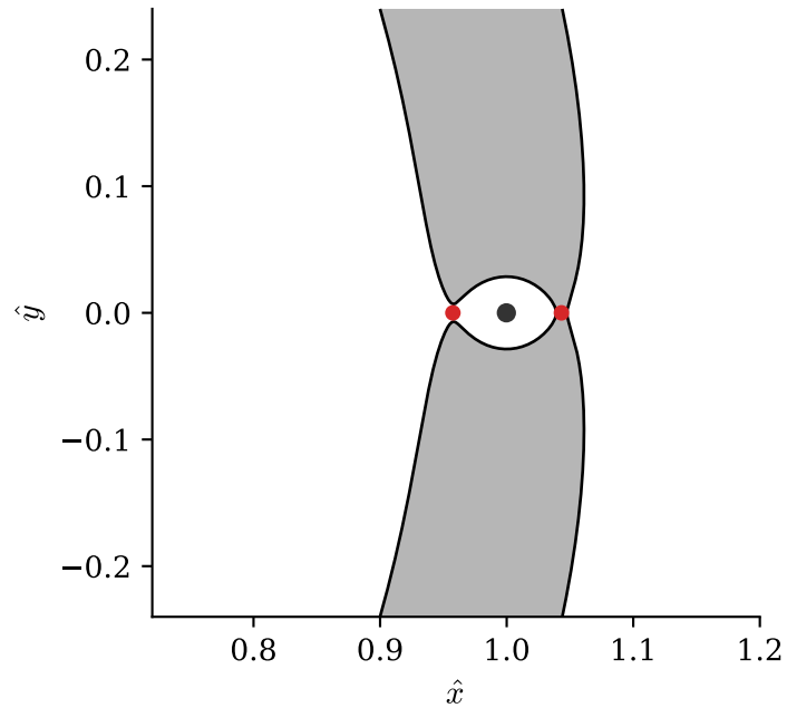
Saturn-Titan \mu=0.0002366 , JC=3.015608
